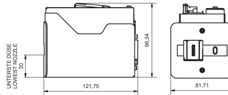
Dimension drawing technical data
